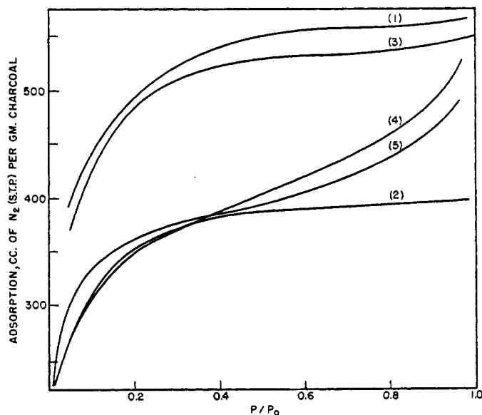
FIG. 32. Adsorption of nitrogen at -195^{\circ}\text{C}. as a function of treatment of the charcoal with chlorine. (1) Untreated CWSN 196 B1X; (2) after chlorine adsorption at 200^{\circ}\text{C}. and evacuation at room temperature; (3) after evacuation at 100^{\circ}\text{C}. ; and (4) and (5) after evacuation at 200^{\circ}\text{C}.
