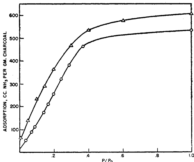
FIG. 31. Adsorption isotherm for ammonia at -46^{\circ}\text{C}. on a sample of CWSN 19 TUC 742 (circles) and on a sample of this charcoal after it had been subjected to surface oxidation by free oxygen at 400^{\circ}\text{C}. (triangles).
