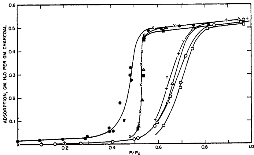
Fig. 9. Water-adsorption and water-desorption isotherms on CWSN 19 as determined by a flow system ( \circ , \bullet ) and by a static system. For the latter, samples were evacuated at 110^{\circ}\text{C} . ( + , \times , and Y for adsorption, desorption, and resorption, respectively); 500^{\circ}\text{C} . ( \triangle and \blacktriangle for adsorption and desorption); and 900^{\circ}\text{C} . ( \square , \blacksquare , \square — for adsorption, desorption, and resorption).
