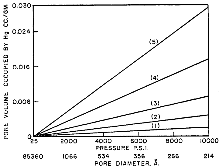
FIG. 24. Pore-size distribution as determined by Ritter and Drake (47, 134) by the high-pressure mercury method for five different silica-alumina gel catalysts.
