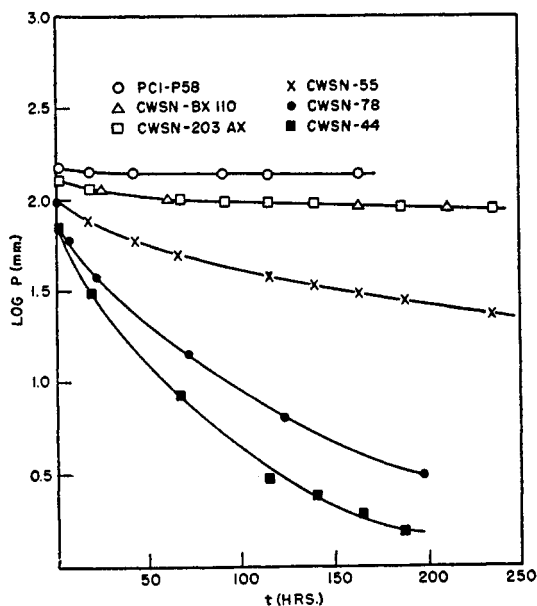
FIG. 28. Rate of oxygen chemisorption at 25°C. by charcoal samples
