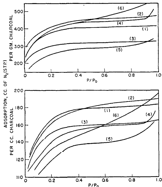
FIG. 26. Nitrogen isotherms showing pore alterations on charcoal CWSN S5 as follows:
